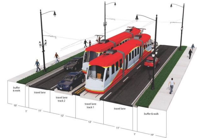
Alternative 2: Median Running Typical Section
